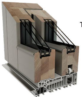
Window thermal insulation Ratio ~1.0 Uw
