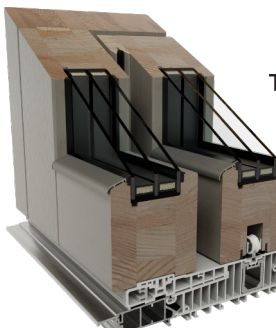
Window thermal insulation Ratio ~0.76 Uw
