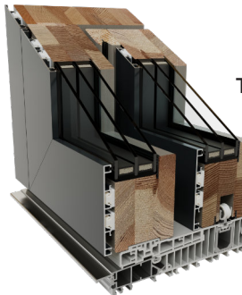
Window thermal insulation Ratio ~1.0 Uw
